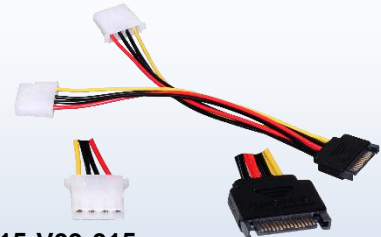
Y15-V03-015 (15 Pin SATA Male to 2 IDE Splitter Female Power Cable 15cm) x1
