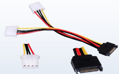
Y15-V03-015 (15 Pin SATA Male to 2 IDE Splitter Female Power Cable 15cm) x2
