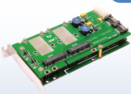
MS2M-4 (Quad mSATA to SATA RAID Adapter) x1
