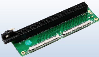
P30F PCIe x16 slot (edge) x1
