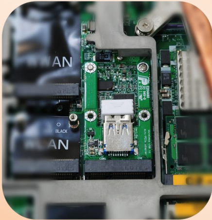
MiniCard slot (Full Size) Max USB device body size:
