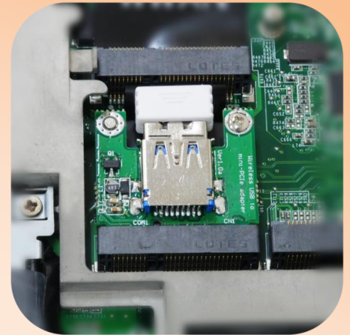
MiniCard slot (Half Size) * After Extra Full-size extensions removed. Max USB device body size:
