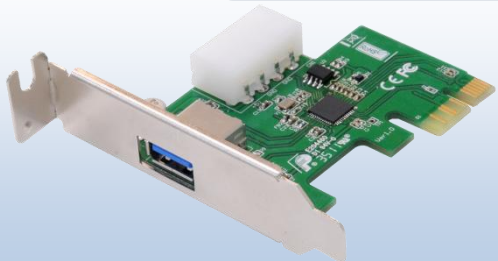
PP1U ( USB3.0 HOST to PCIe Adapter ) x1
