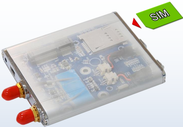
USBMS-E (Wireless USB Mini Card Adapter ver1.2) x1 with SMA IPX cable x2
